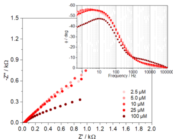
Figure 5: Impedance spectra of chitosan/graphene oxide (2.5%) modified electrode for glucose measurement represented in Nyquist and (inset) Bode plot
